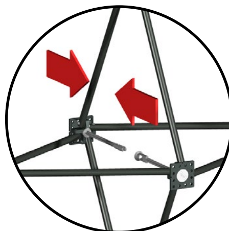
Locking detail 4
